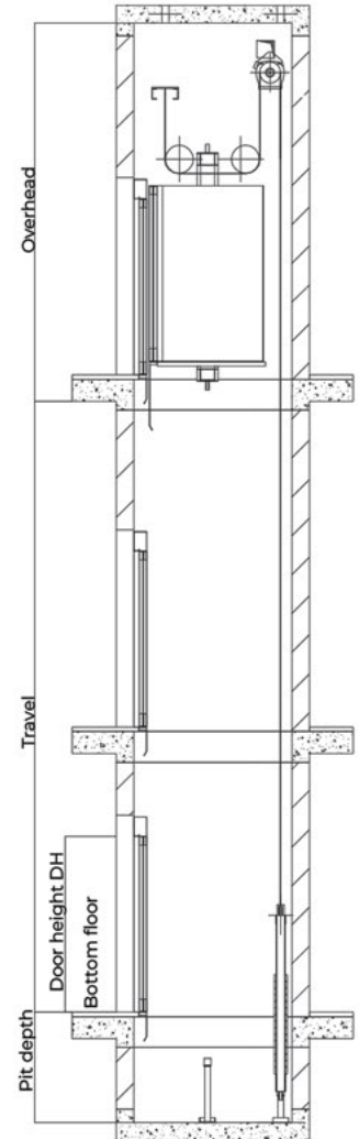
Hoistway section
