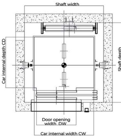
Shaft layout drawing
