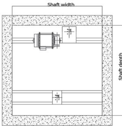
Overhead floor layout drawing
