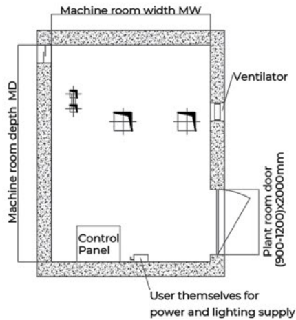
Machine room layout drawing
