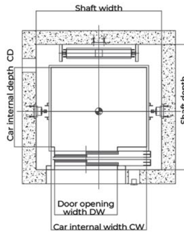
Shaft layout drawing
