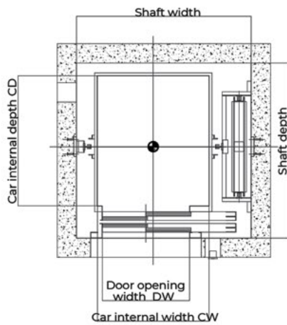
Shaft layout drawing
