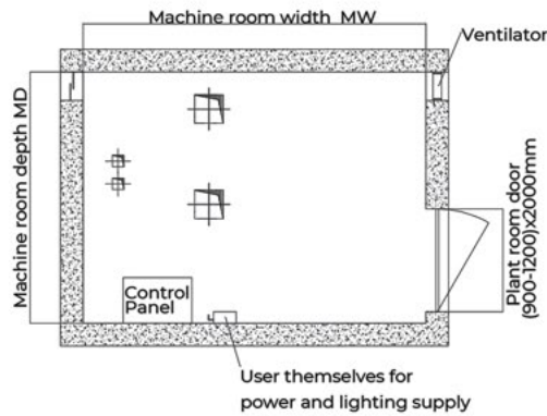
Machine room layout drawing
