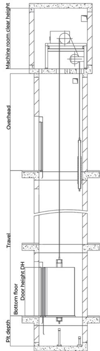
Hoistway section
